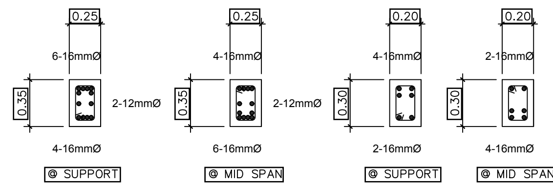
B-1 B-2 SCHEDULE OF BEAMS SCALE: NTS
