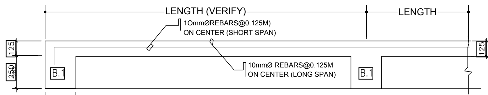
CONCRETE SLAB REINFORCEMENT DETAIL SCALE: NTS
