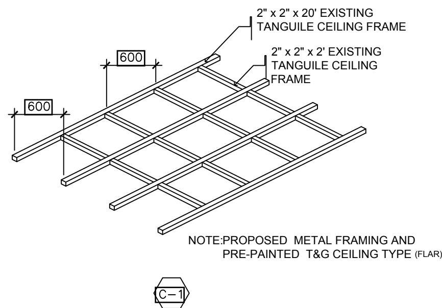
5 CEILING FRAMING SS-5 SCALE: 1:100M
