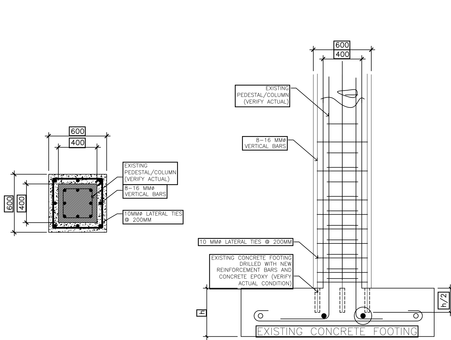
3 TYP. RETROFITTING METHOD SS-5 SCALE: NTS
