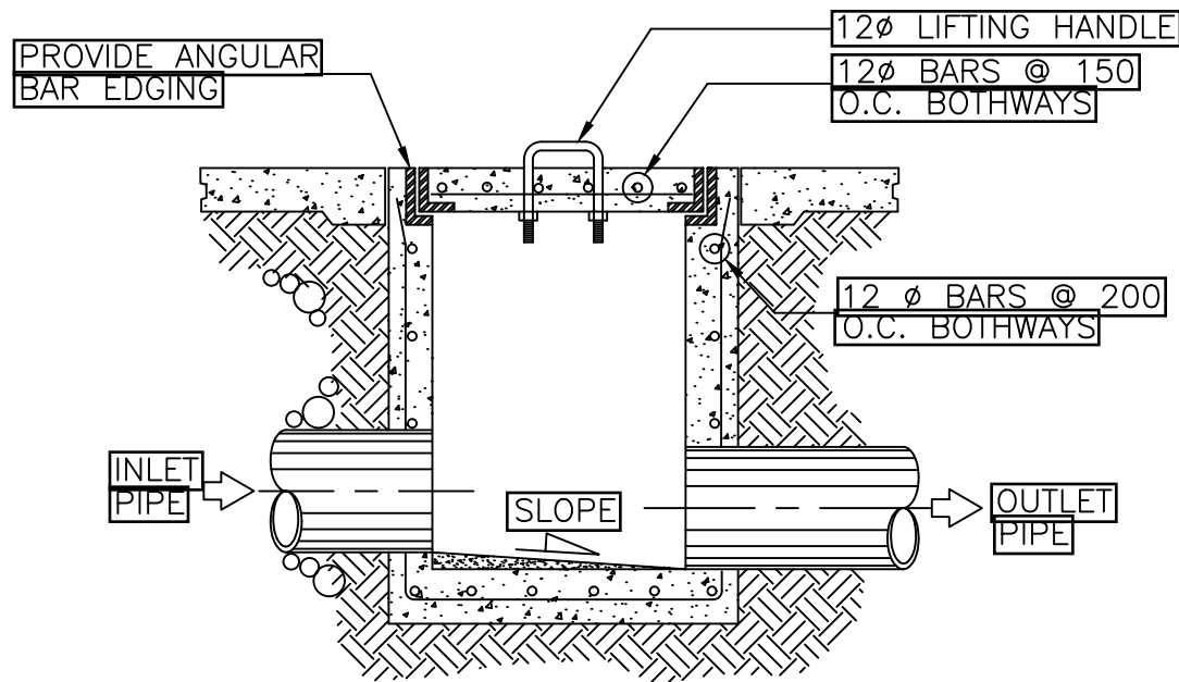
1 P-1 SCALE NTS DETAIL OF CATCH BASIN AND DRAINAGE JUNCTION BOX
