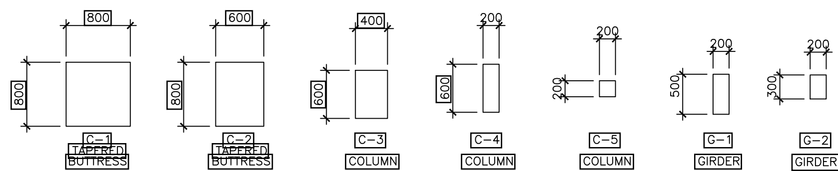
2 TYPICAL COLUMN AND GIDER SIZE SS-5 SCALE: 1:100M
