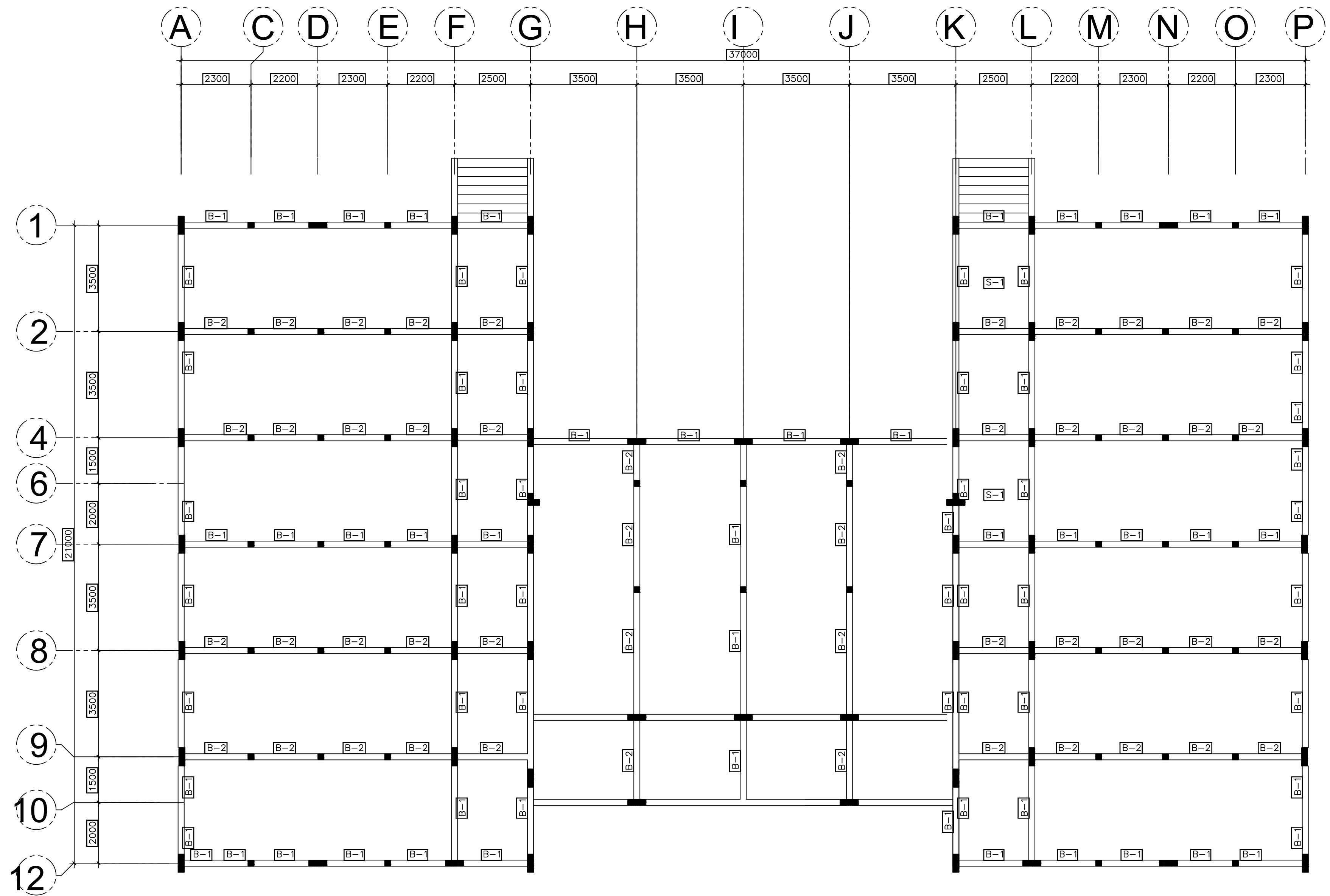
BUILDING 1 1 FLOOR FRAMING PLAN SS-4 SCALE 1:100M
