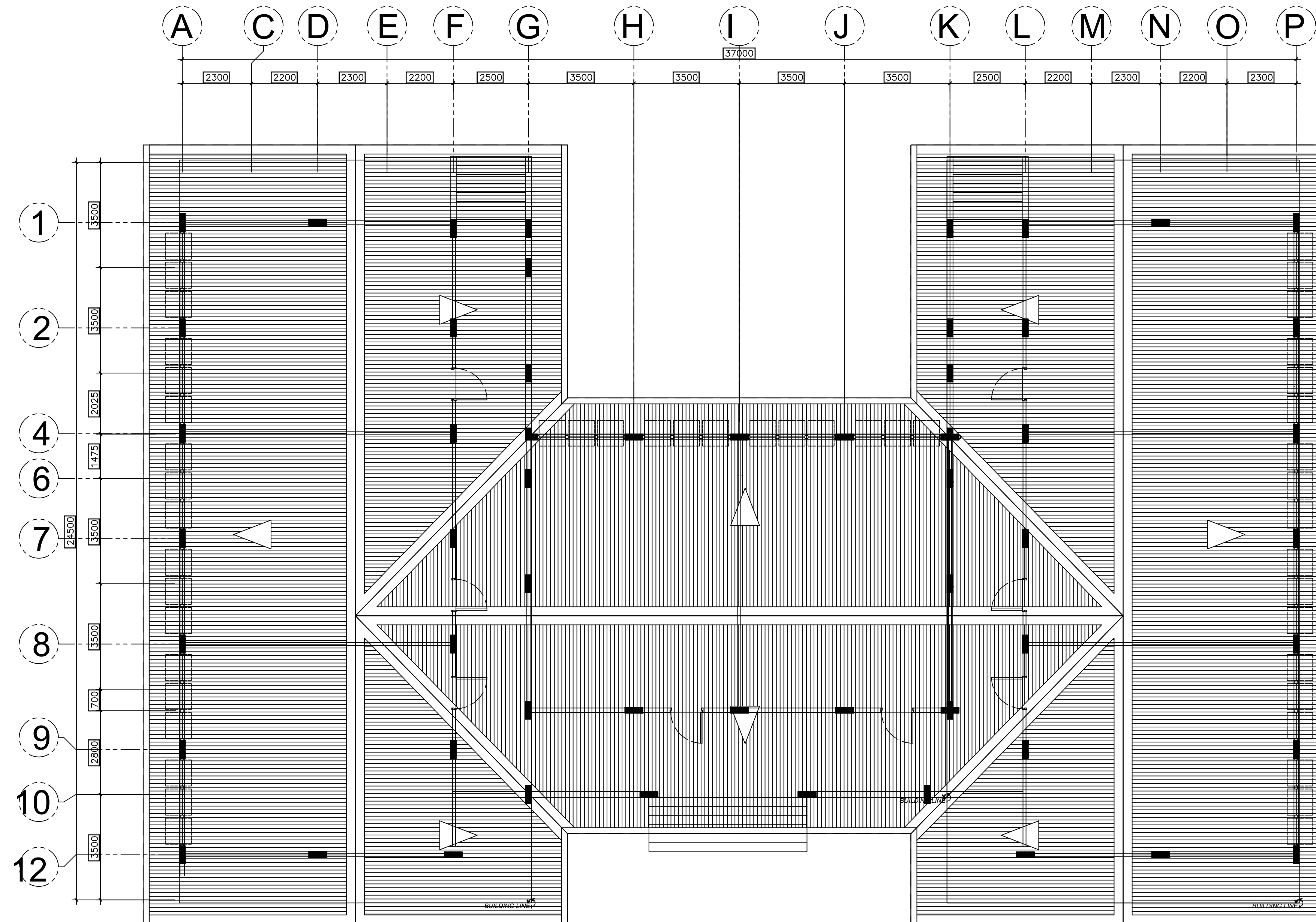
BUILDING 1 ROOF PLAN A-4 SCALE 1:100M
