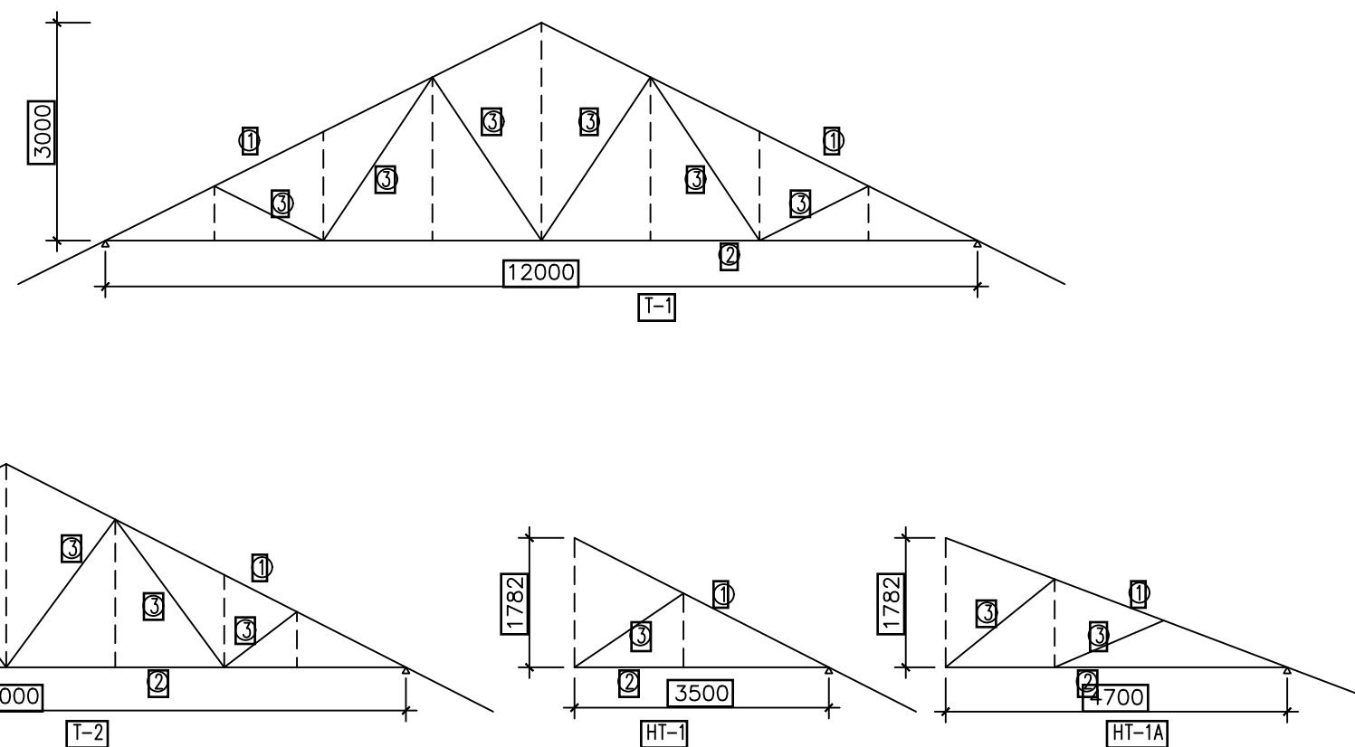
6 TYPICAL TRUSS SCHEDULE SS-5 SCALE: 1:100M
