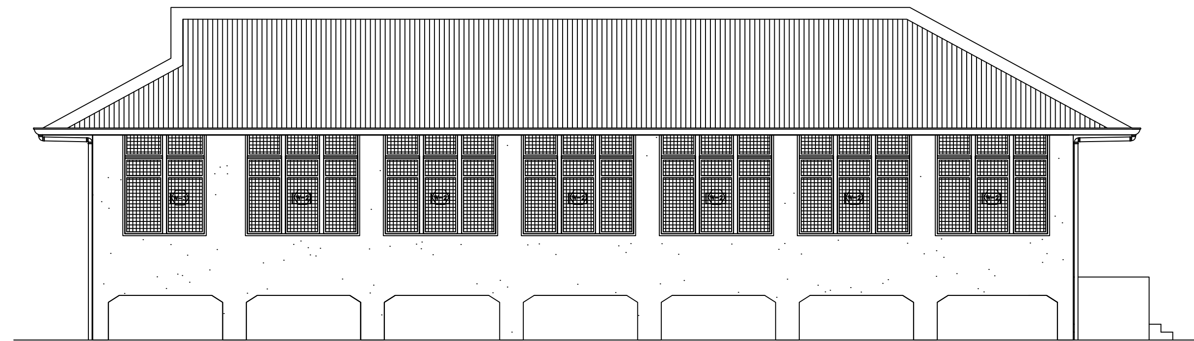
1 BUILDING 1 RIGHT SIDE ELEVATION A-5 SCALE 1:100M
