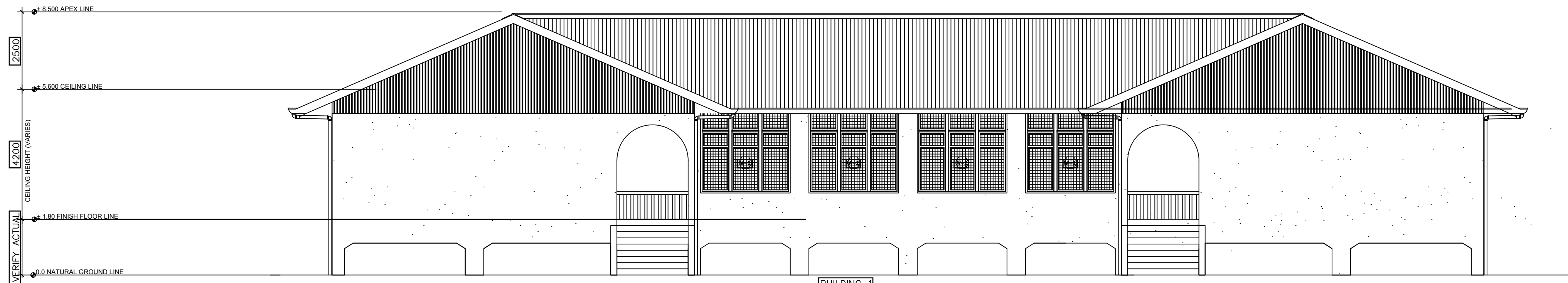
1 BUILDING 1 REAR ELEVATION A-5 SCALE 1:100M
