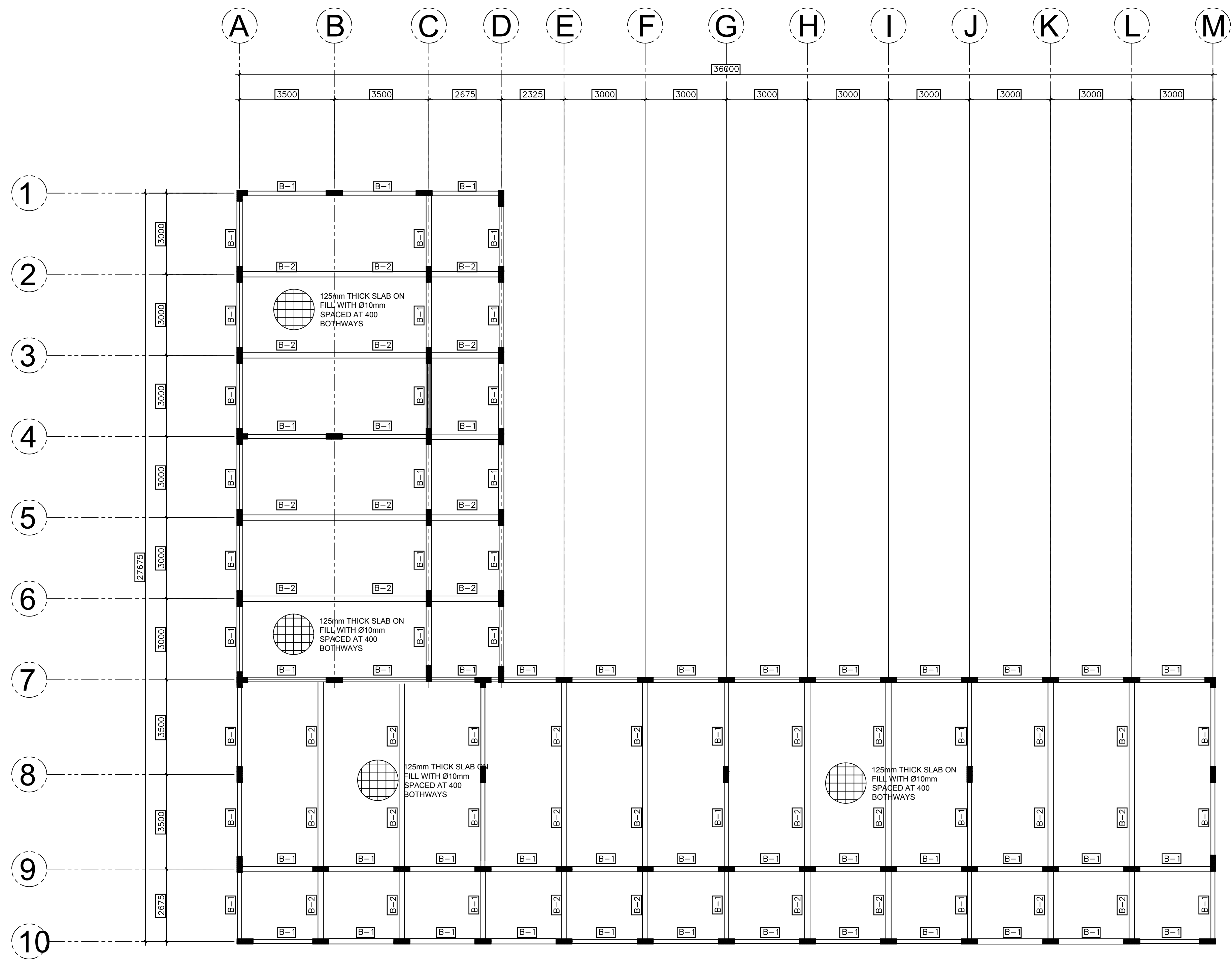
1 FLOOR FRAMING PLAN SCALE 1:100M
