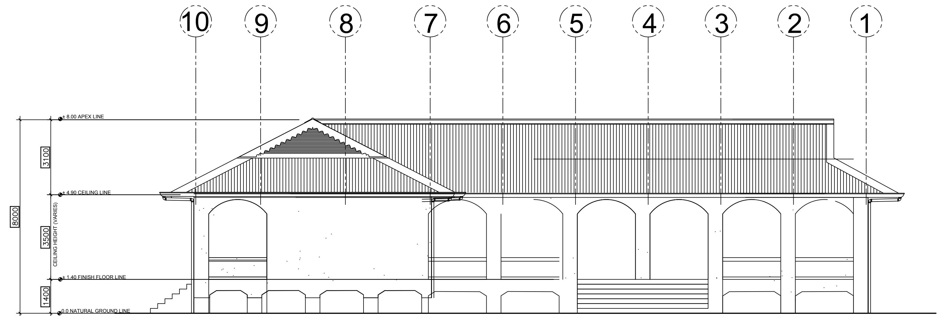
1 RIGHT SIDE ELEVATION A-6 SCALE 1:100M
