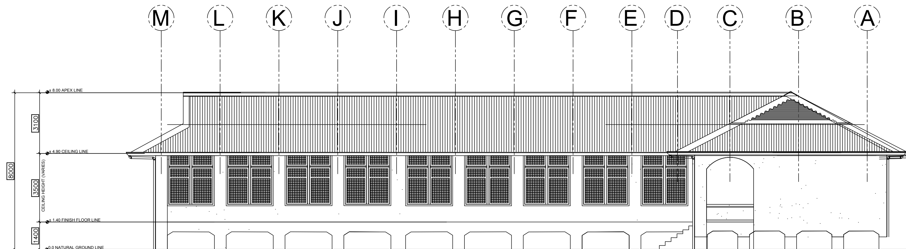
2 REAR ELEVATION A-5 SCALE 1:100M
