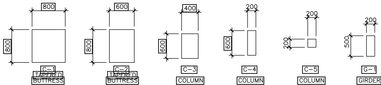
2 TYPICAL COLUMN AND GIDER SIZE S-2 SCALE 1:100M
