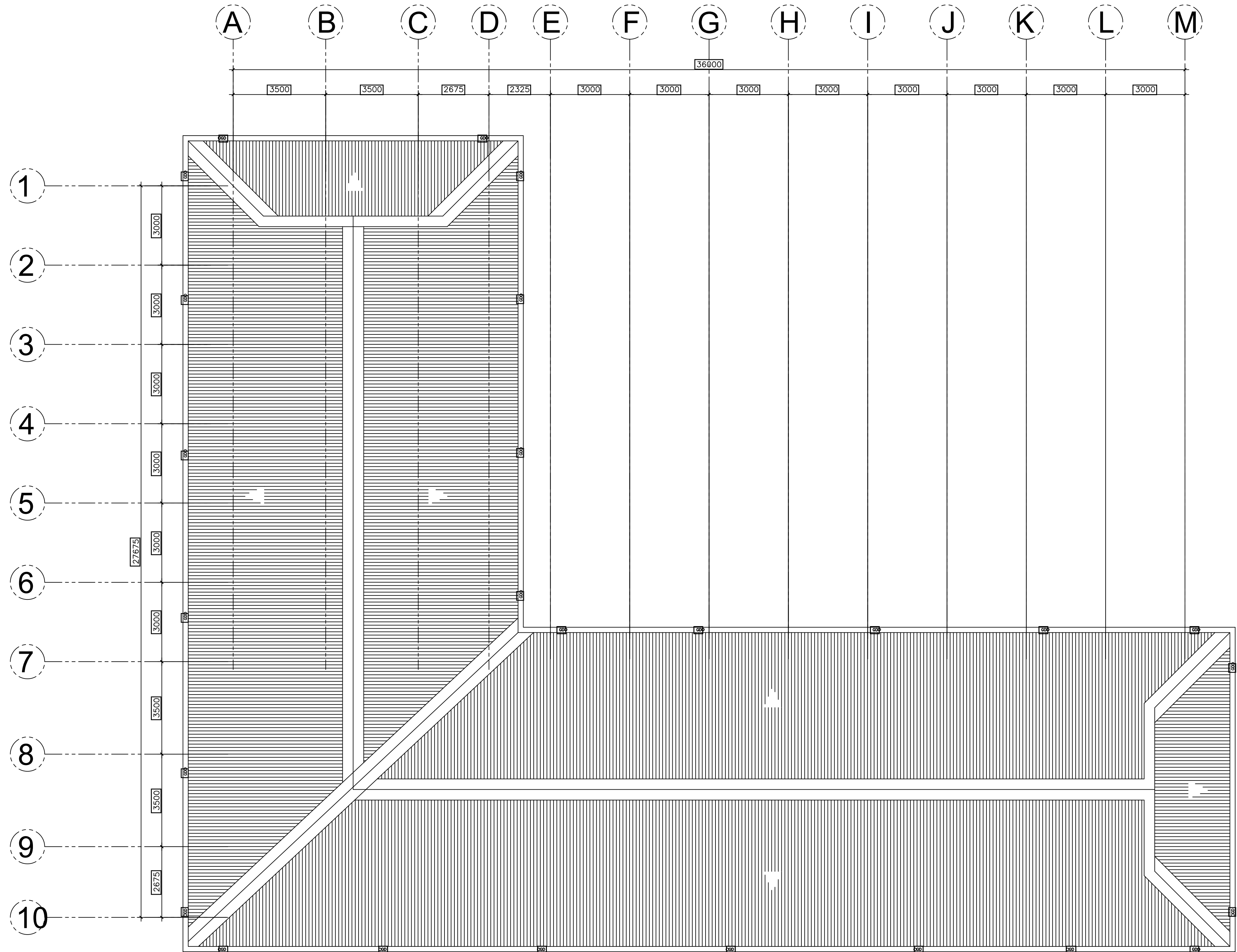
1 ROOF PLAN A-4 SCALE 1:100M
