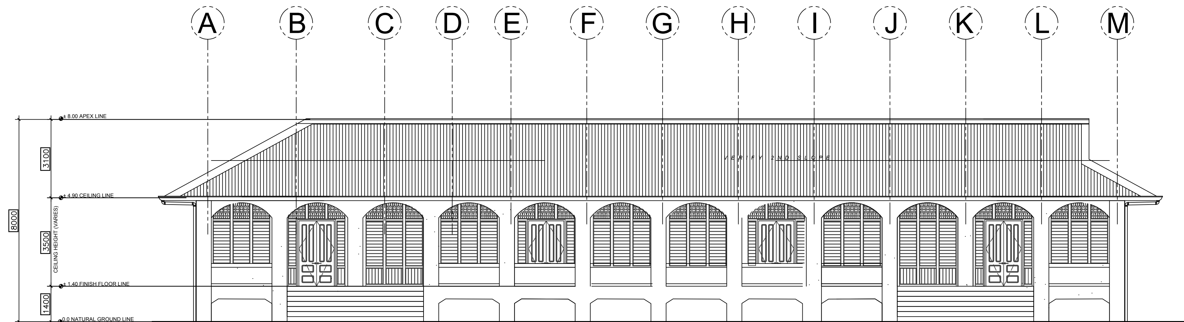
1 FRONT ELEVATION A-5 SCALE 1:100M
