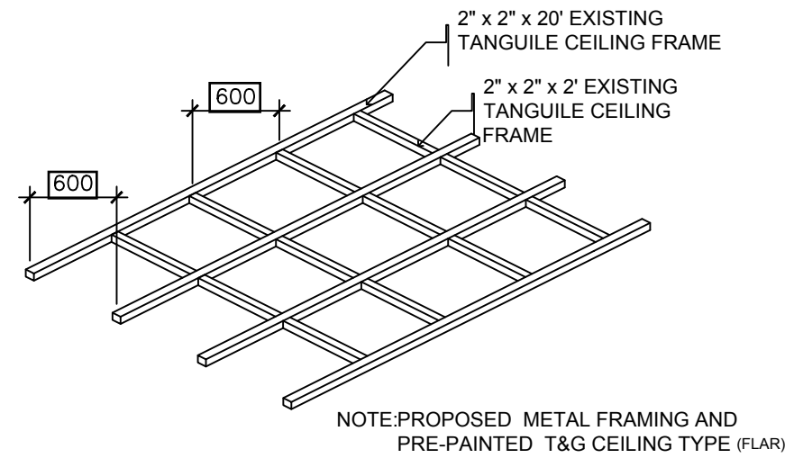
5 CEILING FRAMING DETAIL S-2 SCALE 1:100M
