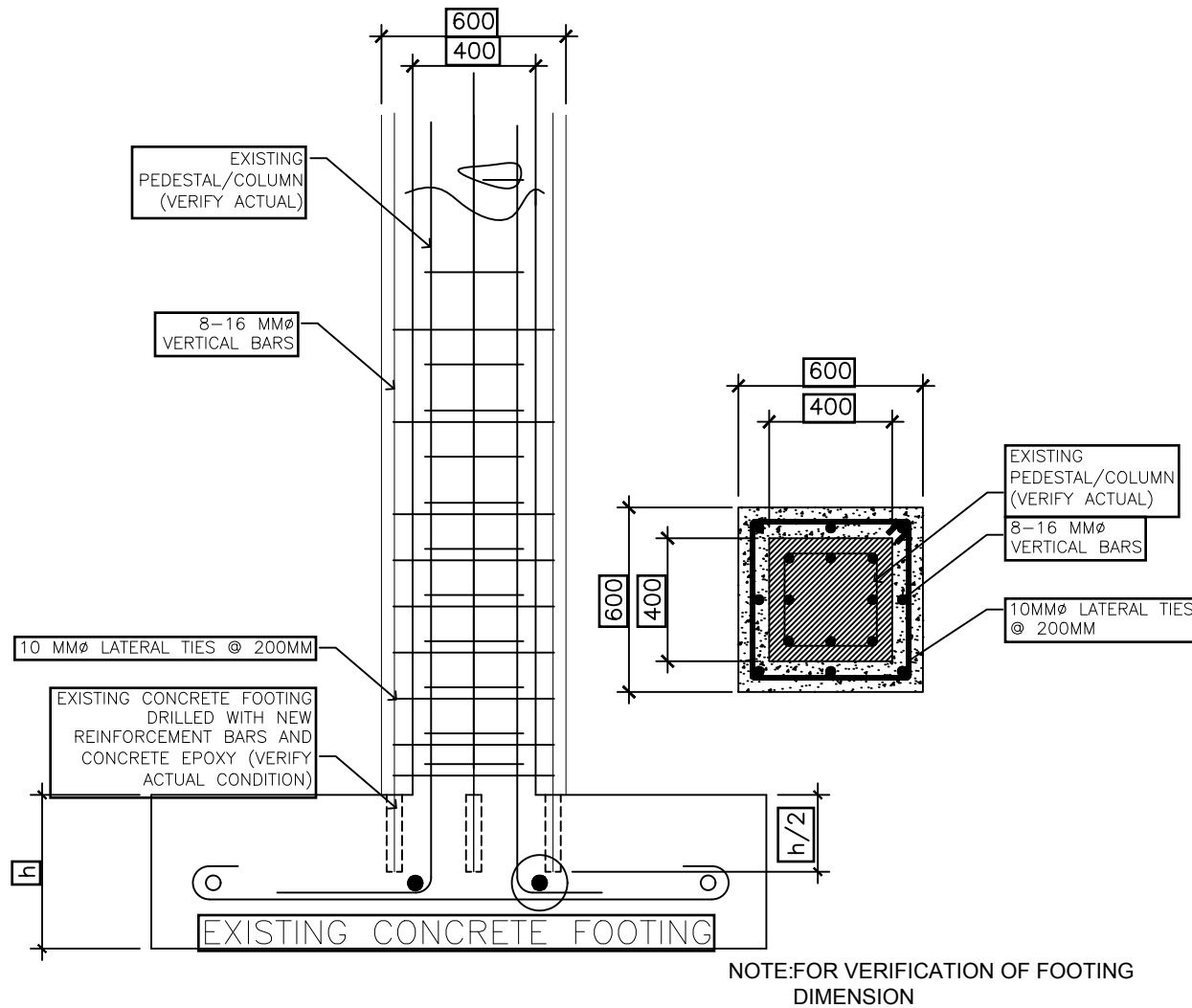
1 TYP. RETROFITTING METHOD S-2 SCALE 1:100M
