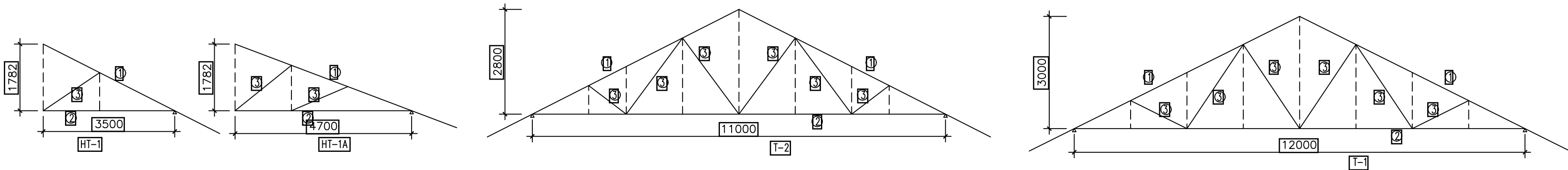
3 TYPICAL TRUSS SCHEDULE S-2 SCALE 1:100M
