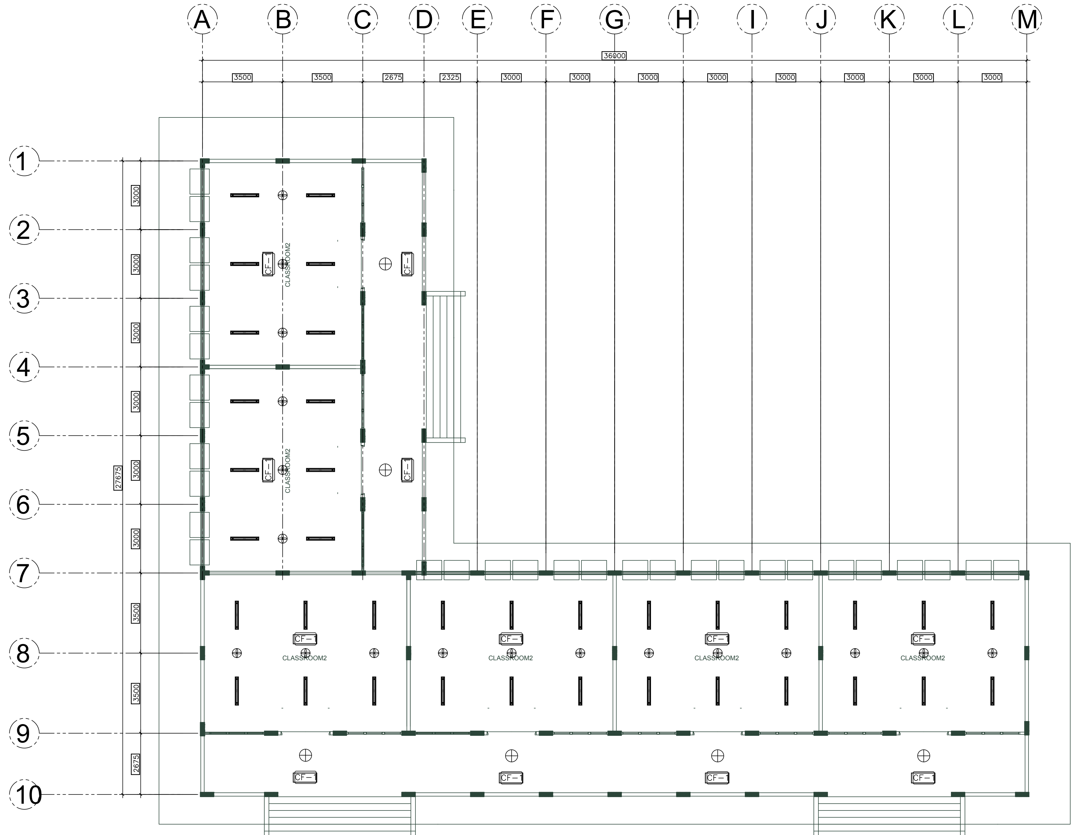
1 REFLECTED CEILING PLAN A-3 SCALE 1:100M
