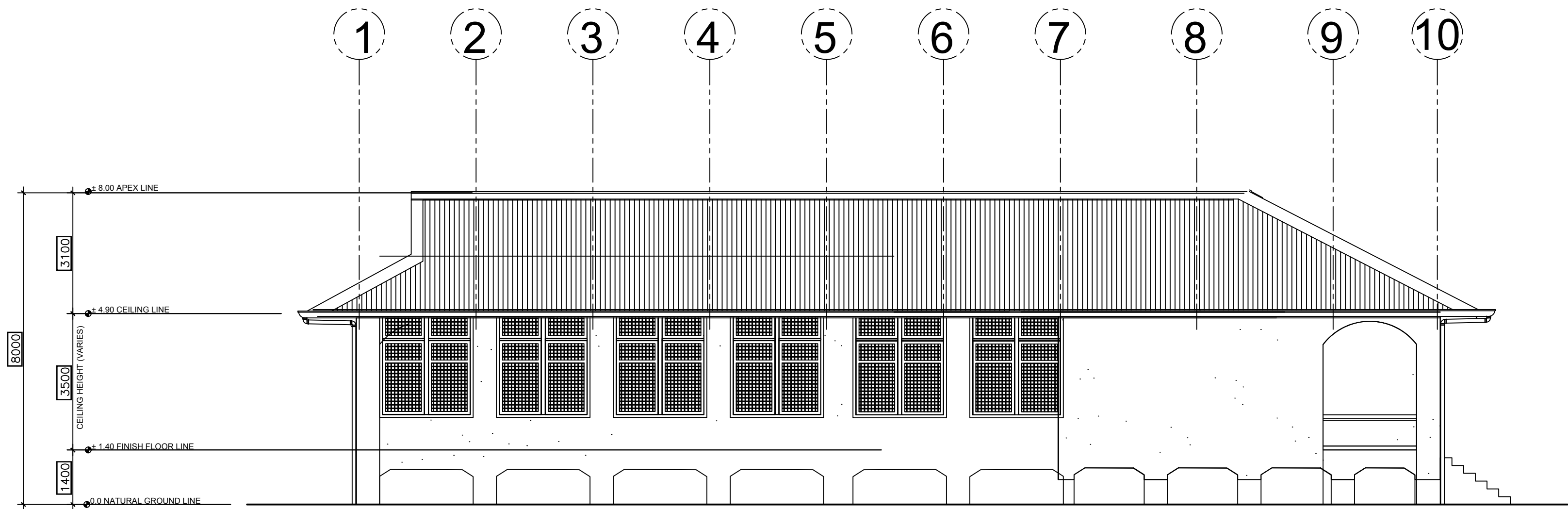
2 LEFT SIDE ELEVATION A-6 SCALE 1:100M
